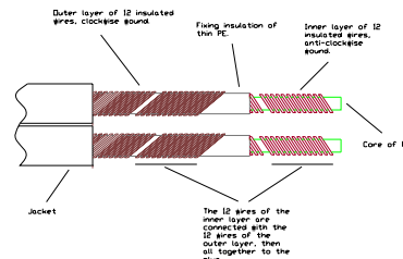
Supra Sword Patented Bifilar Wound Litz
